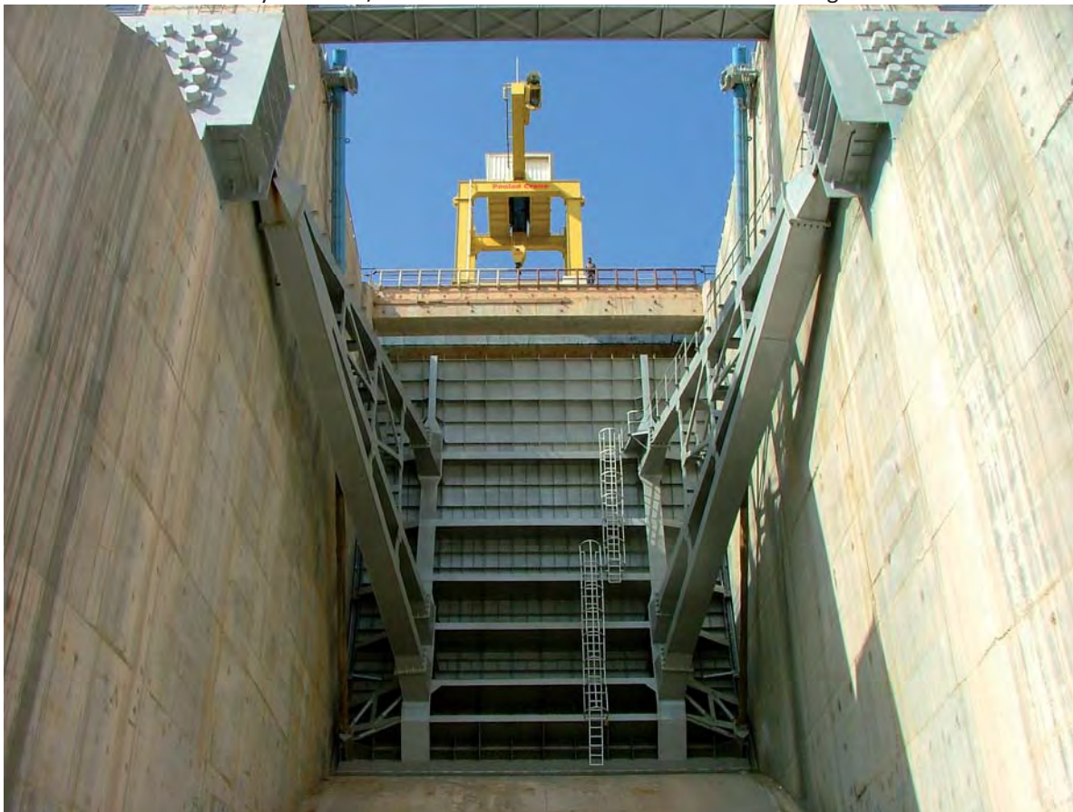
Dam Crane –Gantry Crane 40/3.2 Ton – with 8 meters outreach access for gate maintenance
