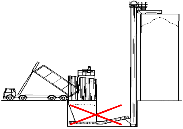
Underground Hopper
